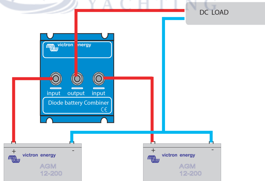
System with two batteries
